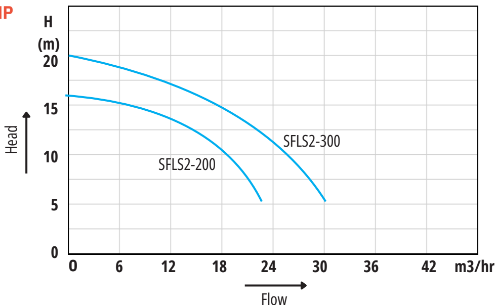
Performance curve
