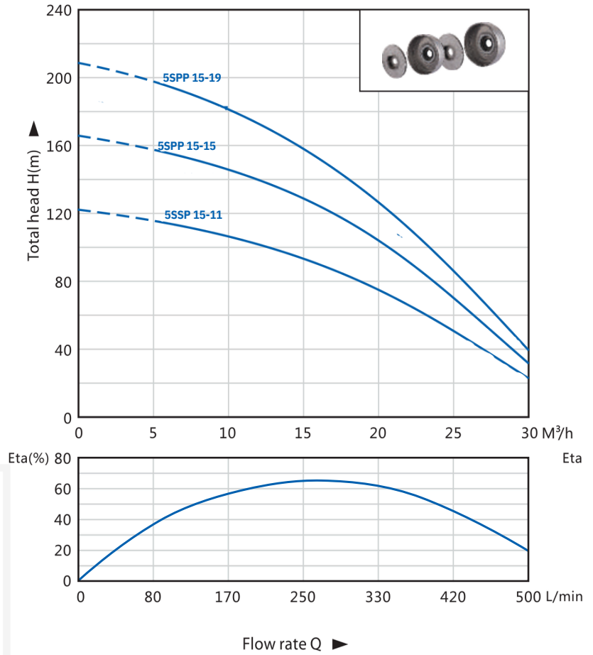
PERFORMANCE CHART AT N=2850RPM
